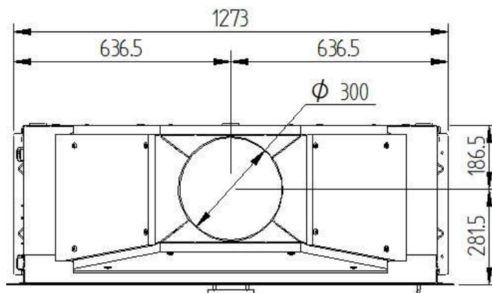
MATAKANA 1200 - OVERALL DIMENSIONS OF THE FIRE
