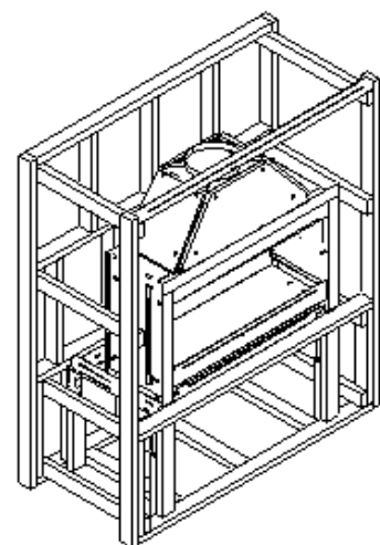
OUTER FRAME WITH BASE FRAME, ANGLE & FIRE
